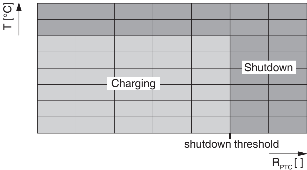
Schematic diagram
