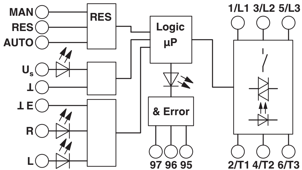
Block diagram
