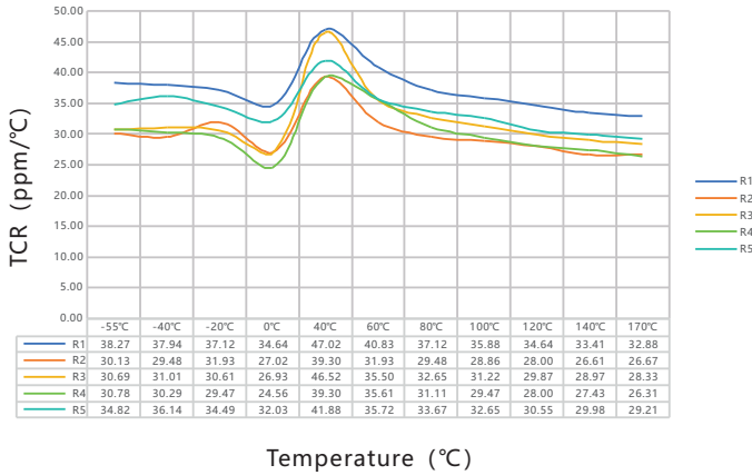
TCR Test Curve -PEWK3920 2.0mΩ
