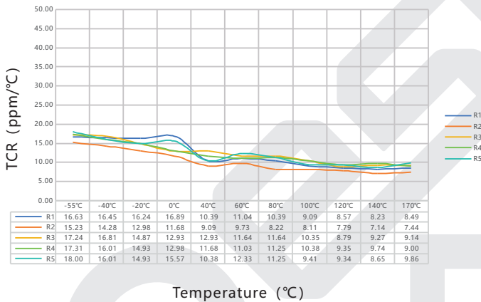
TCR Test Curve -PEWK3920 4.0mΩ
