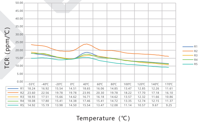
TCR Test Curve -PEWK3920 5.0mΩ
