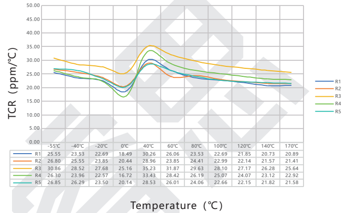
TCR Test Curve -PEWK3920 3.0mΩ
