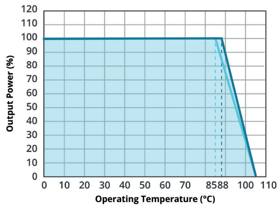
TEMPERATURE DERATING CURVE with heatsink ( V_{in} = 36V )
