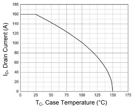
Figure 13. Drain Current vs. T_C
