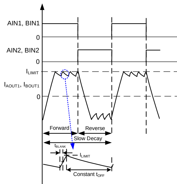
Figure 6: Internal PWM Current Control Waveform
