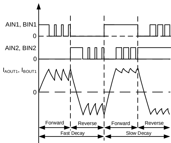
Figure 5: External PWM Current Control Waveform
