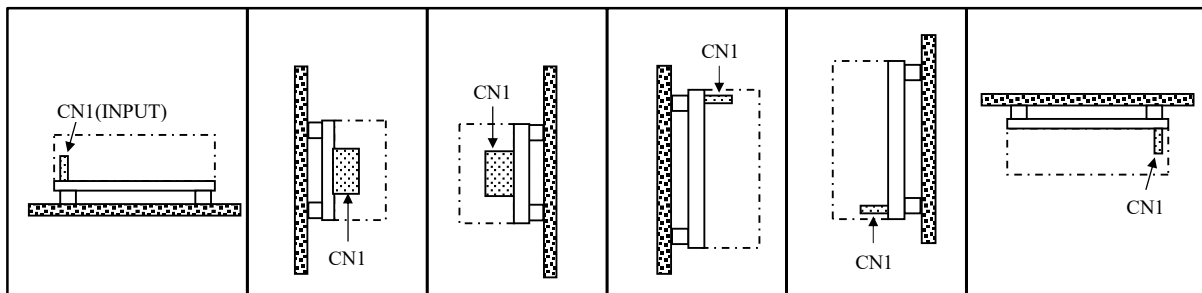
MOUNTING A MOUNTING B MOUNTING C MOUNTING D MOUNTING E MOUNTING F (STANDARD MOUNTING)
