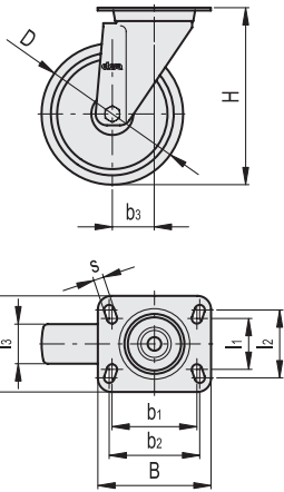
RE.F7-SBL-N
