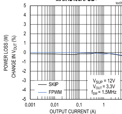
OUTPUT LOAD REGULATION MAX42406AFOB+
