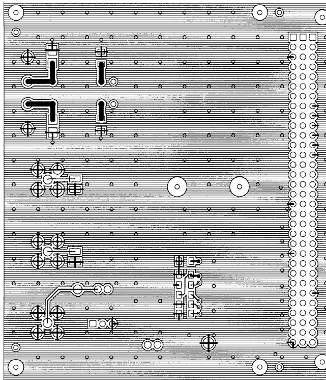
FIGURE 2. PRIMARY SIDE
