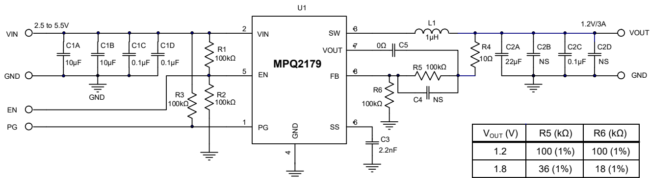
Figure 1: Evaluation Board Schematic
