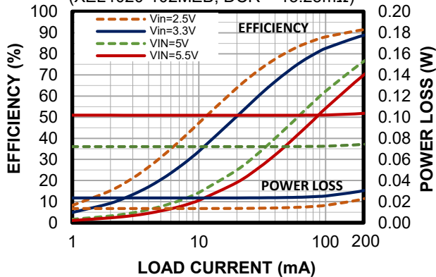
Efficiency vs. Load Current vs. Power Loss (Light Loads)
