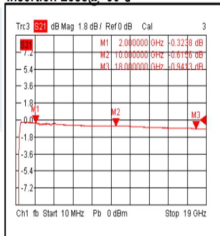
Insertion Loss@+85°C
