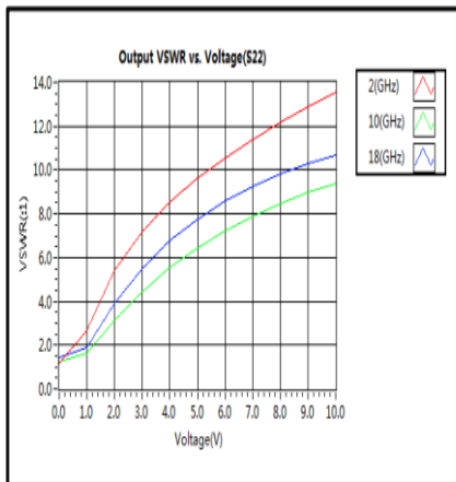
Output VSWR vs. Voltage(S22)
