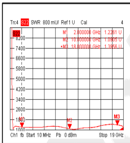
Output VSWR@+85°C
