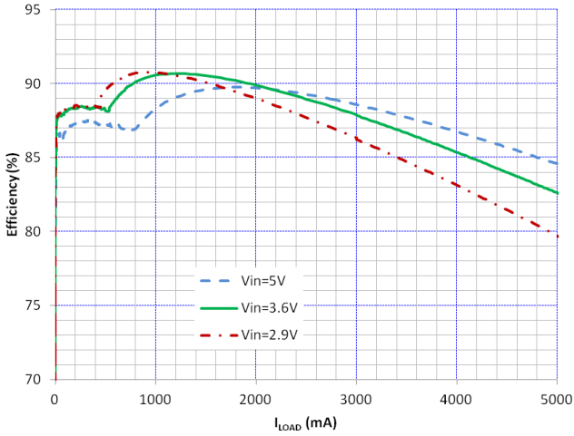
Figure 6. Efficiency vs I_{\text{LOAD}} and V_{\text{IN}} V_{\text{OUT}} = 1.15\text{ V} , SPM5030 Inductor
