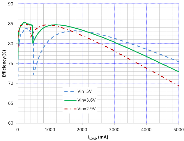
Figure 8. Efficiency vs I_{\text{LOAD}} and V_{\text{IN}} V_{\text{OUT}} = 0.60\text{ V} , SPM5030 Inductor
