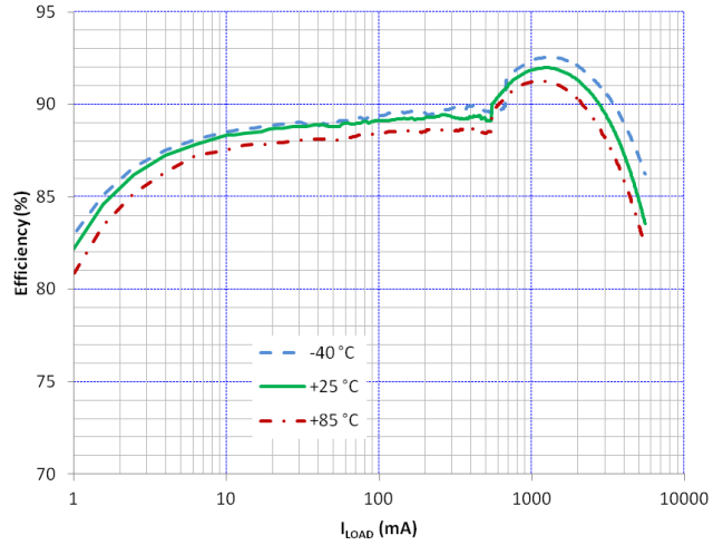
Figure 5. Efficiency vs I_{\text{LOAD}} and Temperature V_{\text{OUT}} = 1.39375\text{ V} , SPM5030 Inductor
