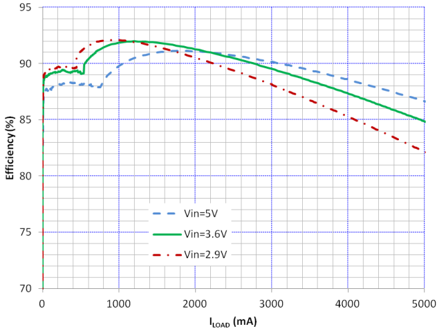
Figure 4. Efficiency vs I_{\text{LOAD}} and V_{\text{IN}} V_{\text{OUT}} = 1.39375\text{ V} , SPM5030 Inductor
