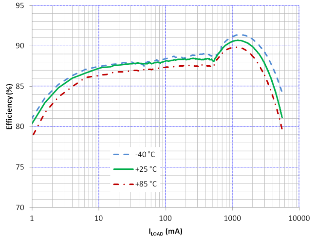
Figure 7. Efficiency vs I_{\text{LOAD}} and Temperature V_{\text{OUT}} = 1.15\text{ V} , SPM5030 Inductor
