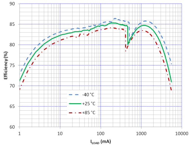
Figure 9. Efficiency vs I_{\text{LOAD}} and Temperature V_{\text{OUT}} = 0.60\text{ V} , SPM5030 Inductor
