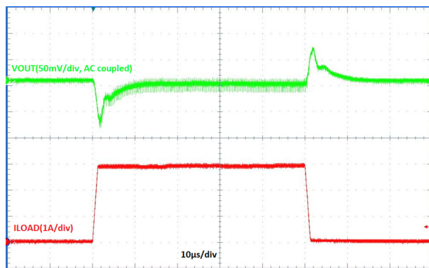
Figure 17. Load Transient (FCCM), I_{OUT} = 10\text{ mA} \leftrightarrow 3\text{ A} , Trise = Tfall = 1\text{ }\mu\text{s}
