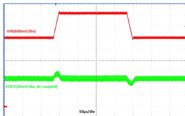
Figure 19. Line Transient, V_{IN} = 3.8\text{ V} \leftrightarrow 5\text{ V} , Slew Rate = 100\text{ mV}/\mu\text{s} , I_{OUT} = 3\text{ A}
