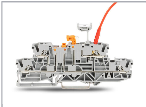
Double-deck, double-disconnect terminal block (Item No. 2002-2951) with group marker carrier (Item No. 2002-160) accommodated in a jumper contact slot and test plug (Item No. 210-136)
