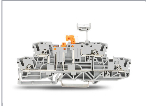
Double-deck, double-disconnect terminal block (Item No. 2002-2951) with group marker carrier (Item No. 2002-160) accommodated in jumper contact slot
