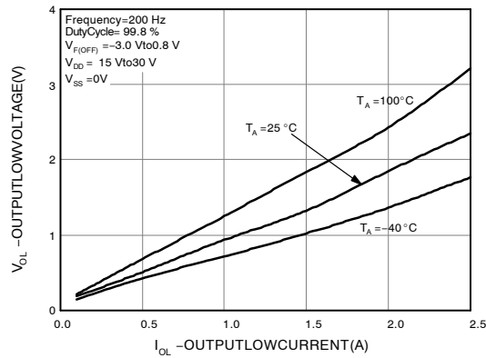
Figure 3. Output Low Voltage vs. Output Low Current
