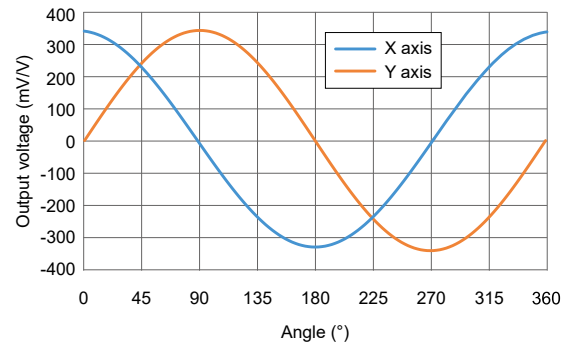
Figure 3. Typical output curve
