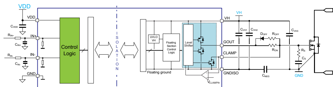
Figure 10. STGAP2SICSA reference schematic for suggested PCB layout
