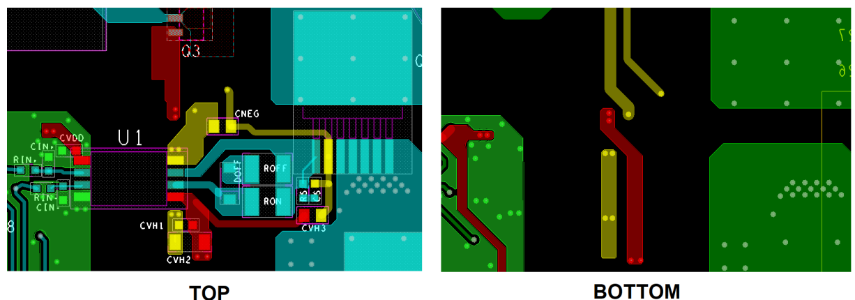
Figure 9. STGAP2SICSA suggested PCB layout: top and bottom
