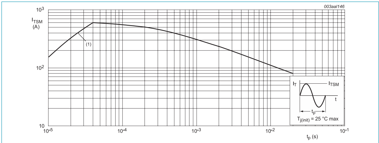
t_p \leq 20 \text{ ms} (1) di_T/dt limit Fig. 5. Non-repetitive peak on-state current as a function of pulse width; maximum values
