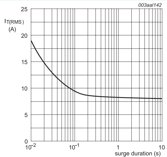
f = 50\text{ Hz} ; T_{mb} = 105\text{ °C} Fig. 2. RMS on-state current as a function of surge duration; maximum values
