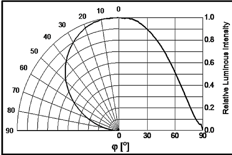
Figure 9. Radiation diagram, Irel = f (Φ)
