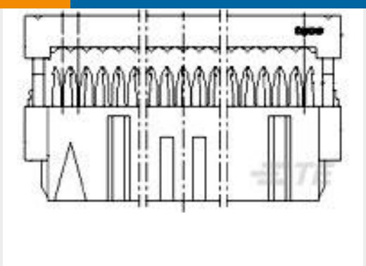
TE Part # 2-215882-0 20 WAY GREY MK II RECP
