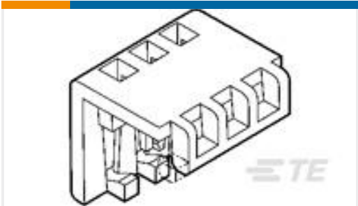
TE Part # 2-643075-3 23P MTA100 MOLDED COVER
