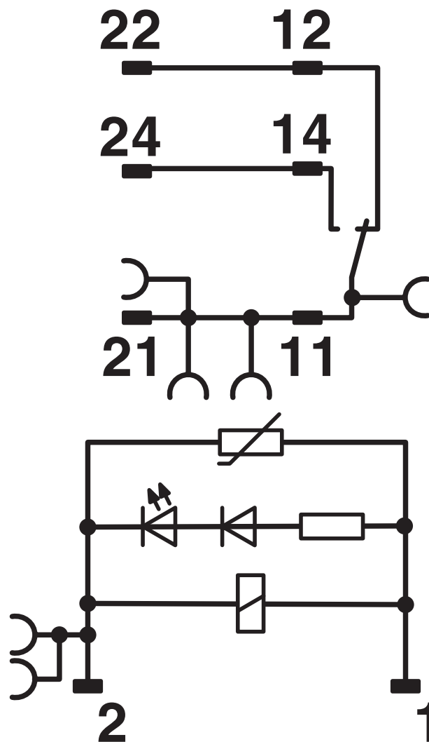
Circuit diagram
