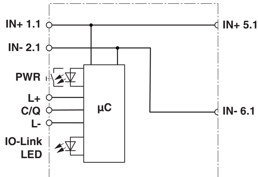
Block diagram
