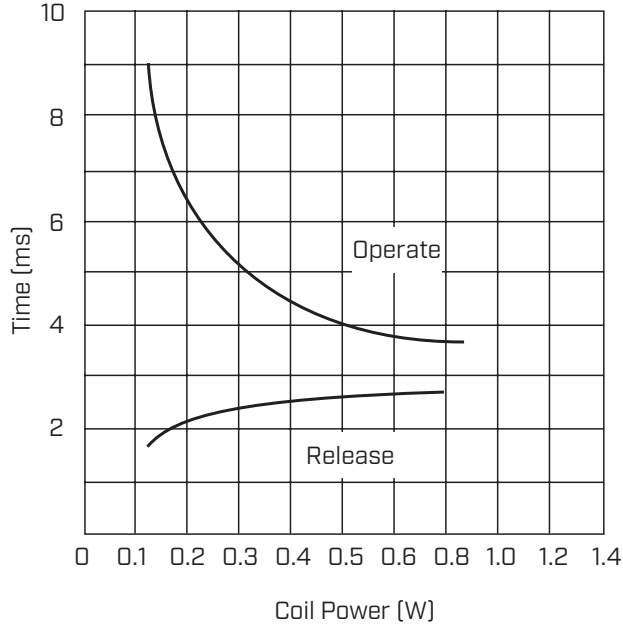
Time Curve
