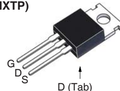
TO-220 (IXTP)
