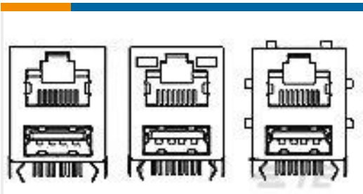
TE Part # 1-1909119-4 VAO, MODULAR JACK, RJ45+USBx1F, W/ LED
