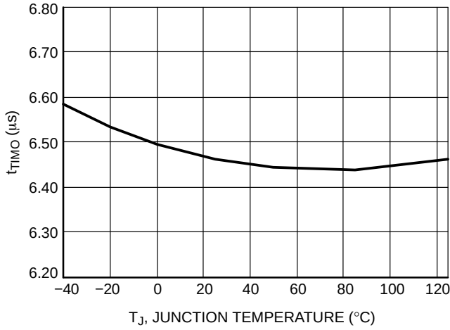
Figure 15. t TIM0 vs. Junction Temperature
