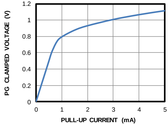
Figure 4: PG Clamped Voltage vs. Pull-Up Current
