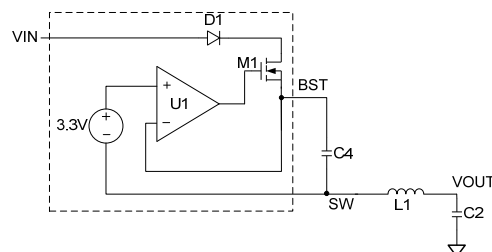
Figure 6: Internal Bootstrap Charging Circuit
