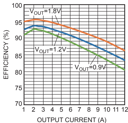
Efficiency Curve
