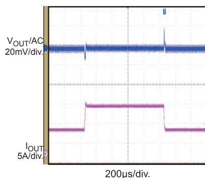
Load Transient
