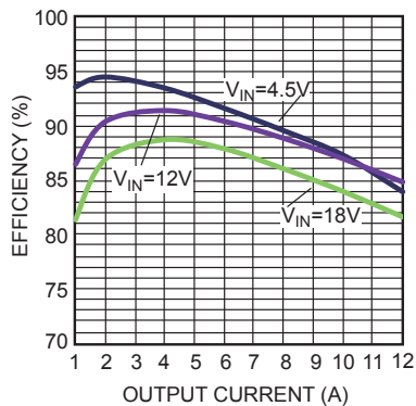
Efficiency vs. Output Current V_{OUT} = 1V , L = 1.5\mu H , DCR = 2.1m\Omega
