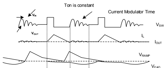
Figure 5: Light-Load Operation
