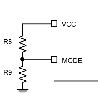
Figure 5: MODE Configuration
