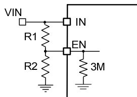
Figure 4 – Adjustable UVLO using EN pin
