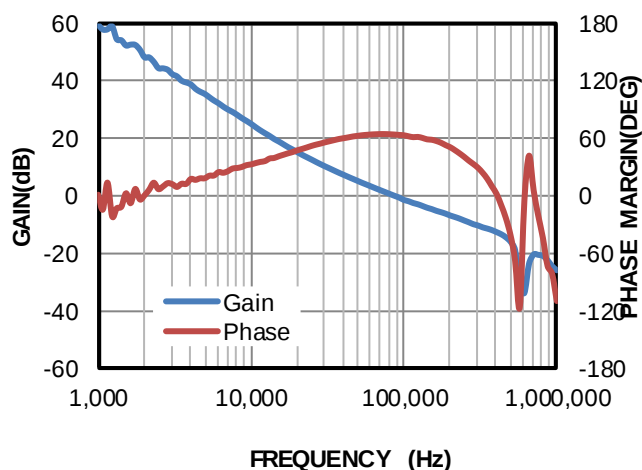
Boode Plot
