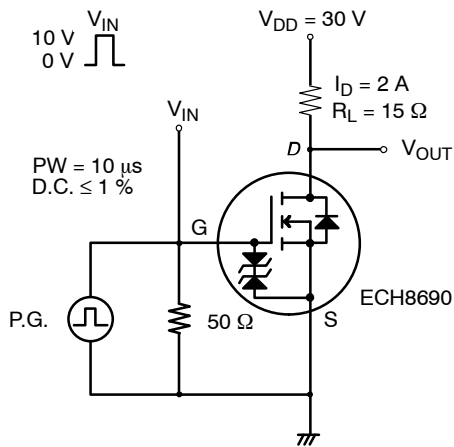
[N-Channel]
