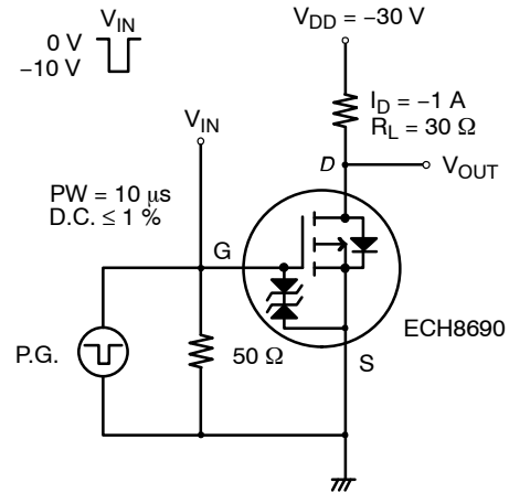
[P-Channel]
