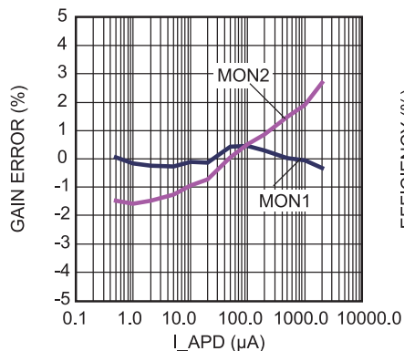
Gain Error vs. APD Current
