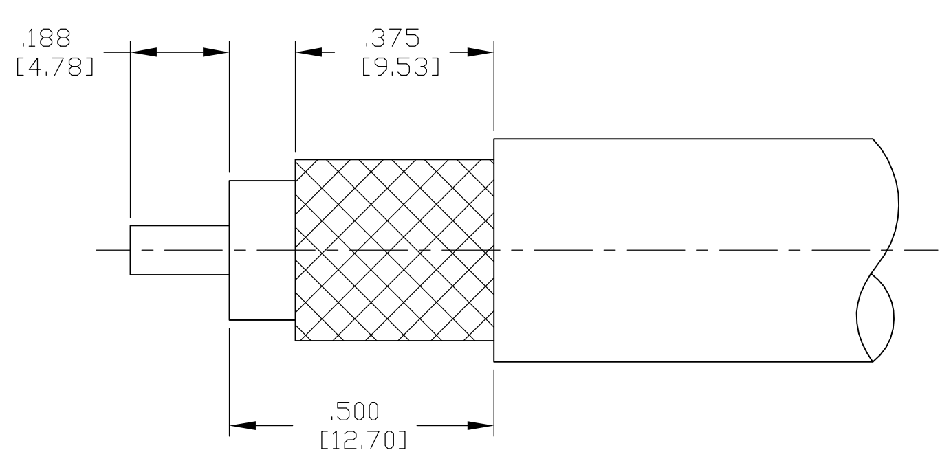
RECOMMENDED STRIP LENGTH SCALE 8:1
