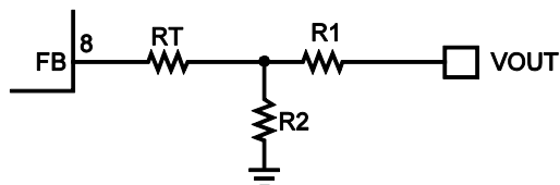
Figure 5: T-Type Network
