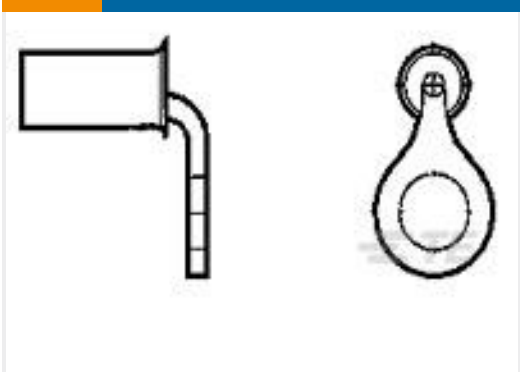
TE Part # 54748-1 TERMINAL R 90 DEG PG 4 1/4
