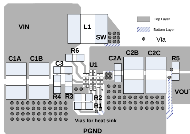
Figure 3: Recommended PCB Layout
