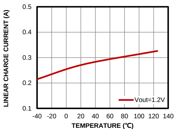
Linear Charge Current vs. Temperature
