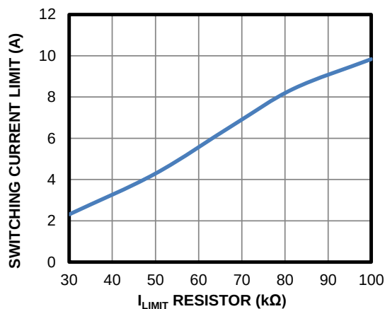
Switching Current Limit vs. I_{LIMIT} Resistor
