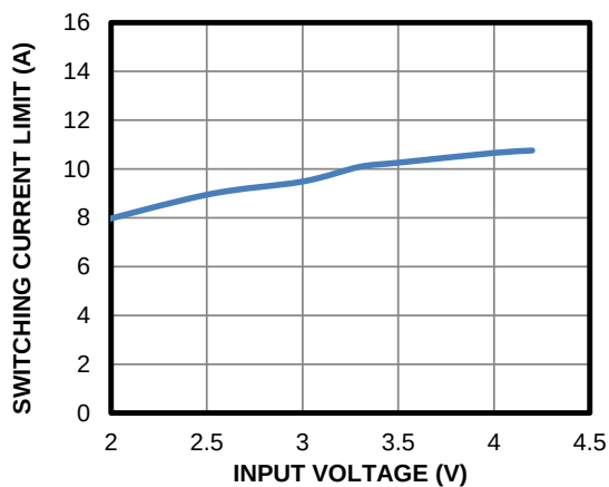
Switching Current Limit vs. Input Voltage
