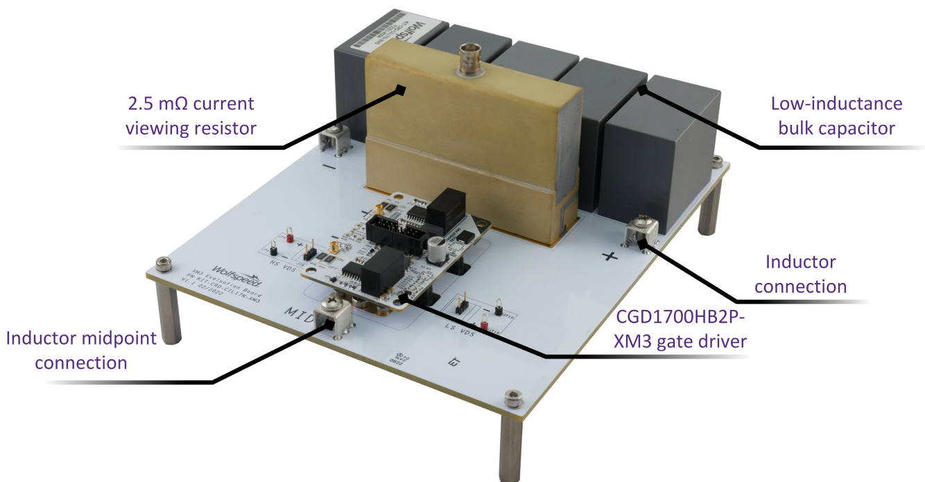
Figure 35: KIT-CRD-CIL17N-XM3 evaluation board
