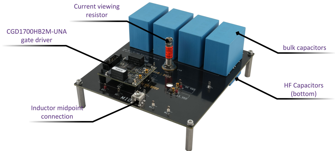
Figure 44: KIT-CRD-CIL12N-DMA CIL Evaluation Board
