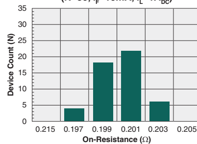
Typical On-Resistance Distribution (N=50, I_F=10\text{mA} , I_L=1\text{A}_{DC} )
