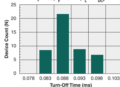
Typical Turn-Off Time (N=50, I_F=10\text{mA} , I_L=1\text{A}_{DC} )
