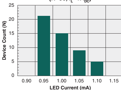
Typical I_F for Switch Dropout (N=50, I_L=1\text{A}_{DC} )
