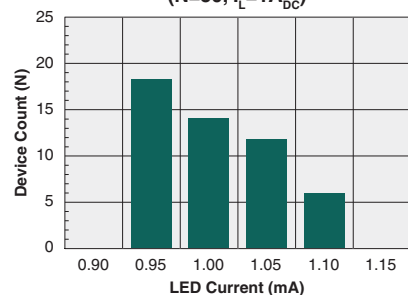
Typical I_F for Switch Operation (N=50, I_L=1\text{A}_{DC} )
