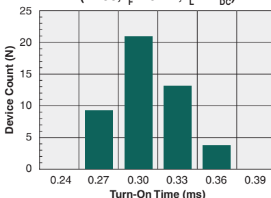
Typical Turn-On Time (N=50, I_F=10\text{mA} , I_L=1\text{A}_{DC} )
