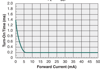
Typical Turn-On Time vs. LED Forward Current ( I_L=1\text{A}_{DC} )
