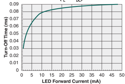
Typical Turn-Off Time vs. LED Forward Current ( I_L=1\text{A}_{DC} )
