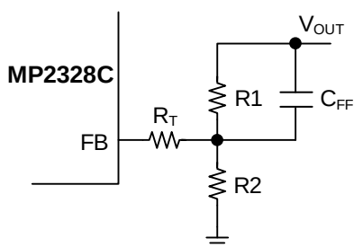
Figure 3: Feedback Network
