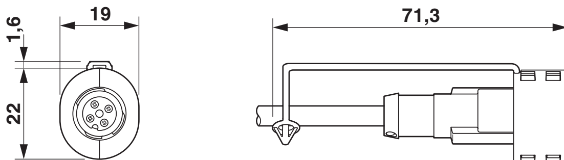
EXCLIP mounted plug
