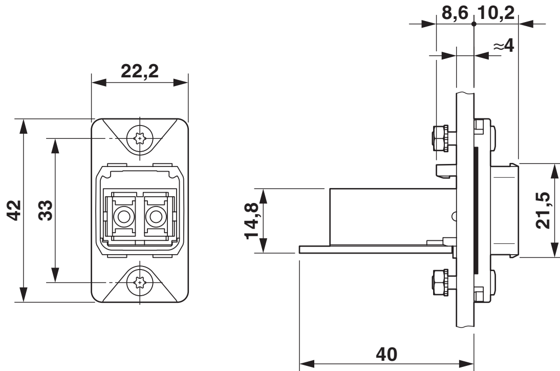
Dimensional drawing
