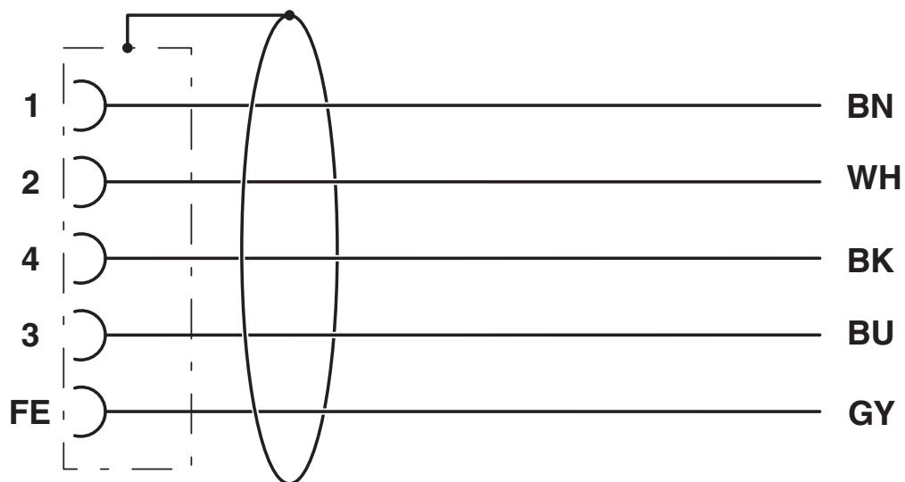
Circuit diagram
