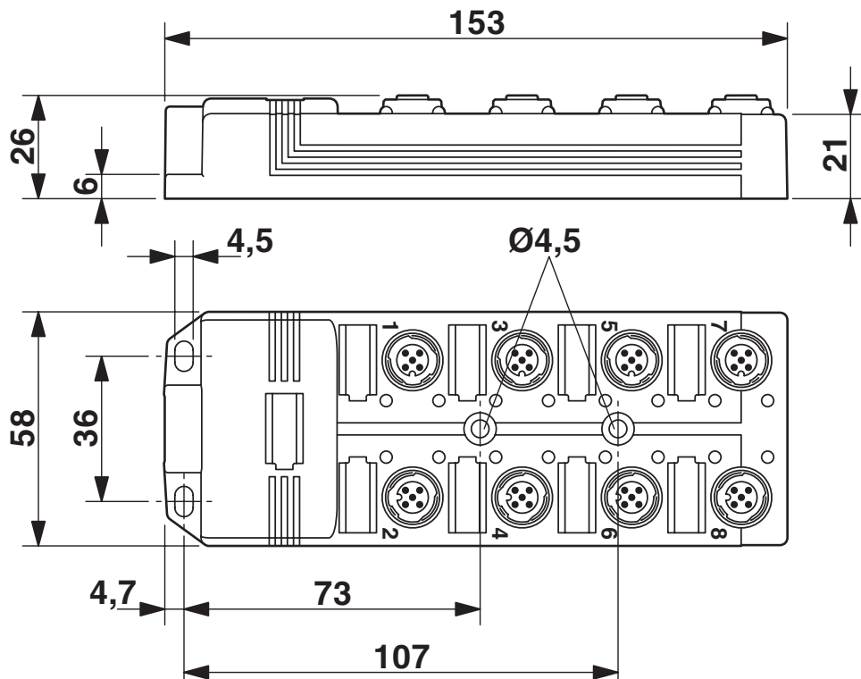
Dimensional drawing
