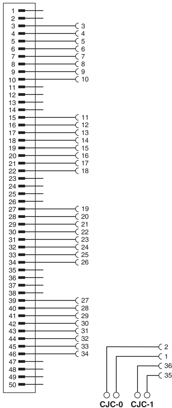
Circuit diagram
