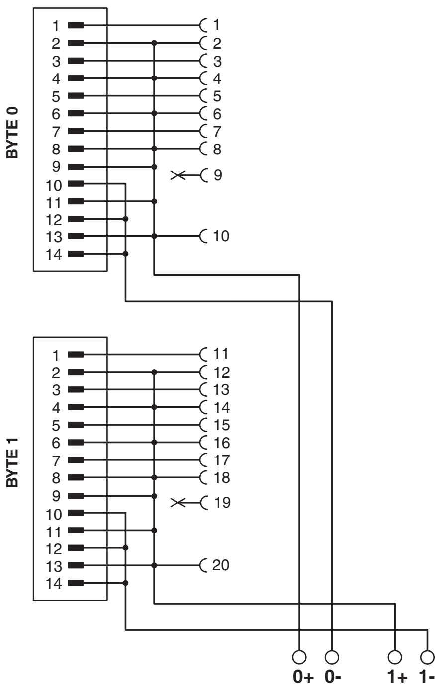
Circuit diagram
