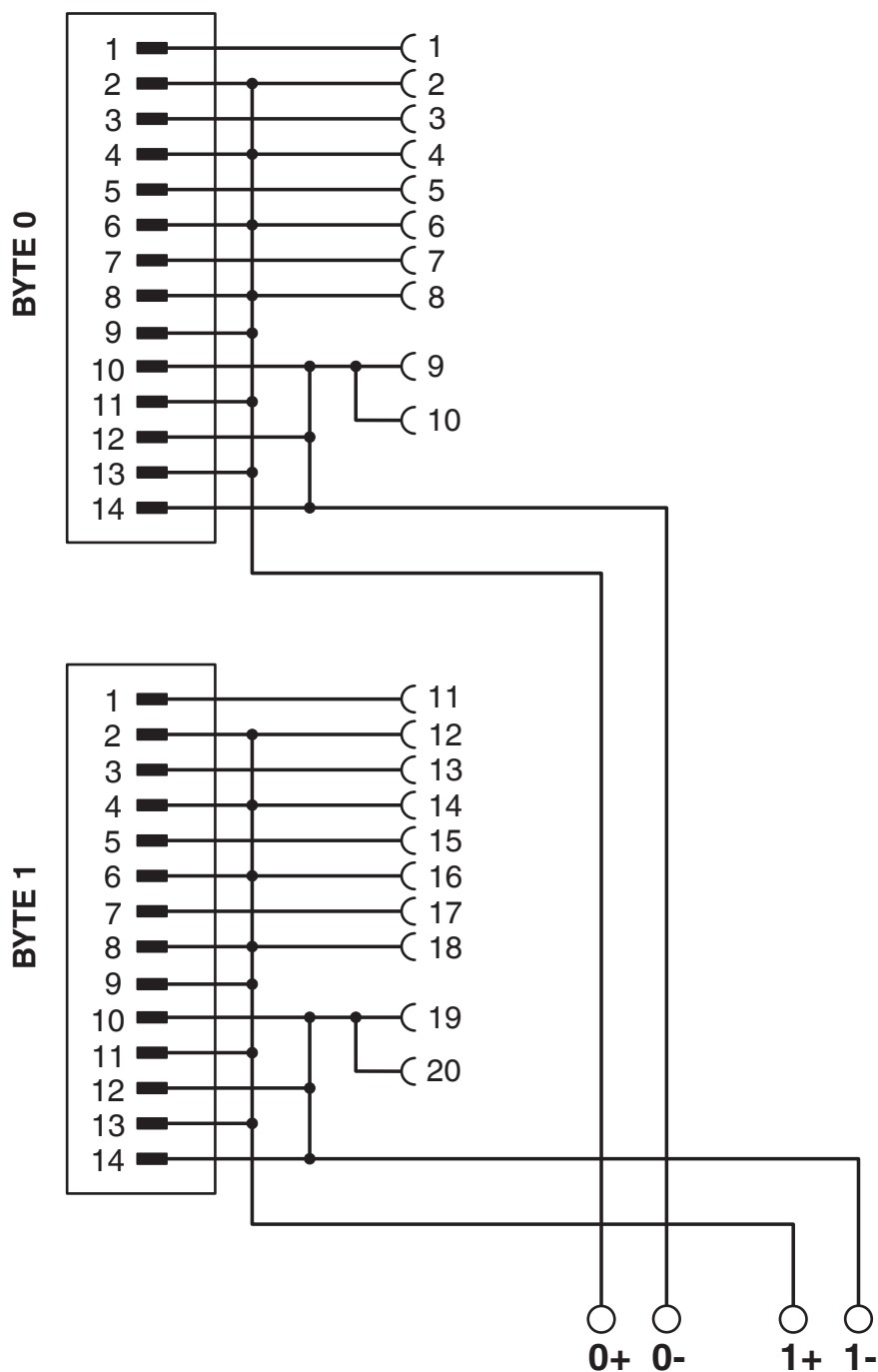
Circuit diagram
