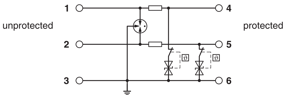
Circuit diagram
